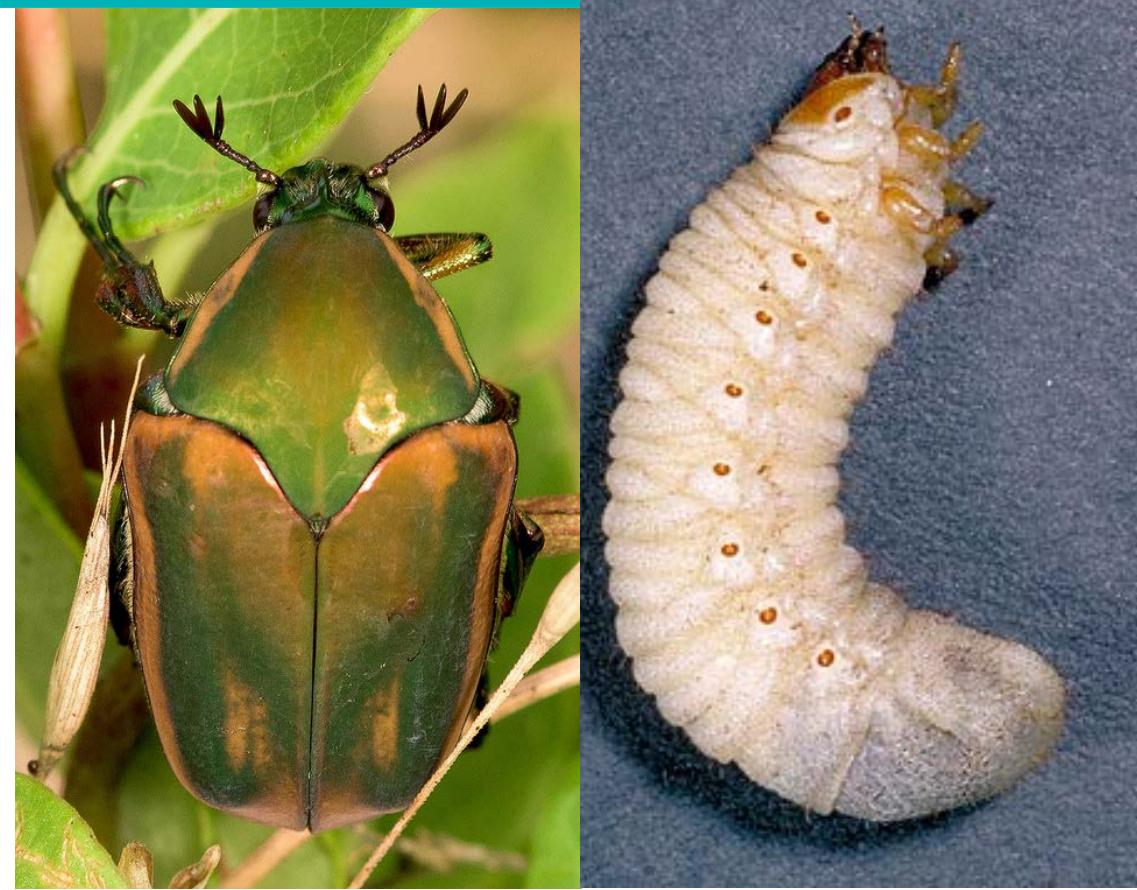
Left: Green June beetle adult; Right: Green June beetle larvae. Photo Cred: Mark Etheridge & P. Shrewsbury
